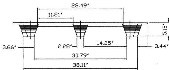
45" END VIEW
