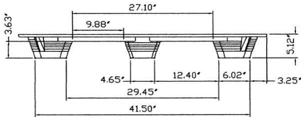
48" END VIEW
