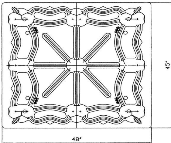
45" END VIEW
