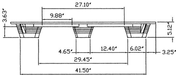
48" END VIEW
