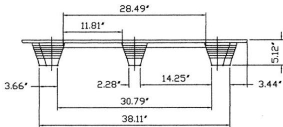
45" END VIEW
