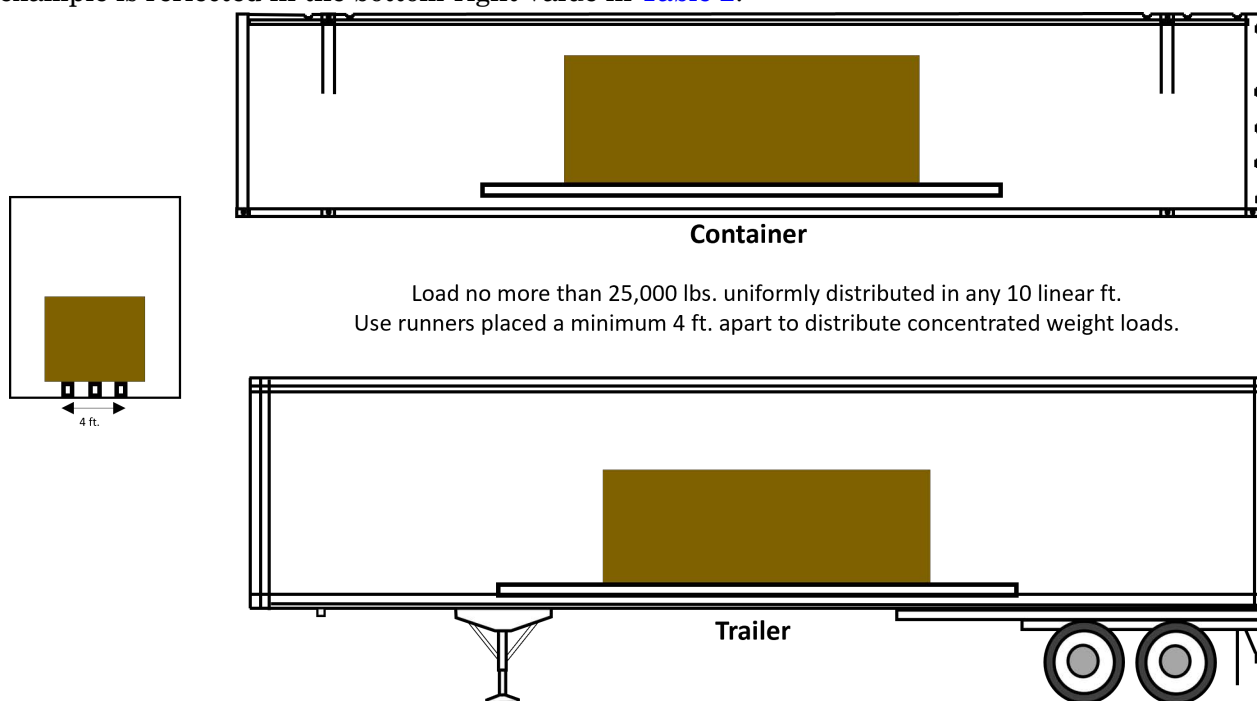
Figure 2: Weight distribution for concentrated weight
