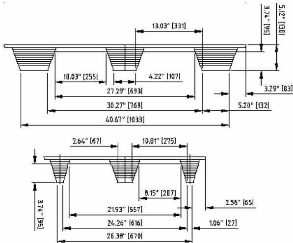
1200mm x 800mm (47.24" x 31.5") PRESSWOOD PALLET
