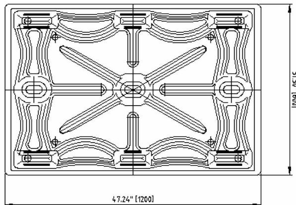
1200mm x 800mm (47.24" x 31.5") PRESSWOOD PALLET
