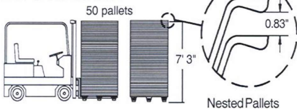
Nested Pallets
