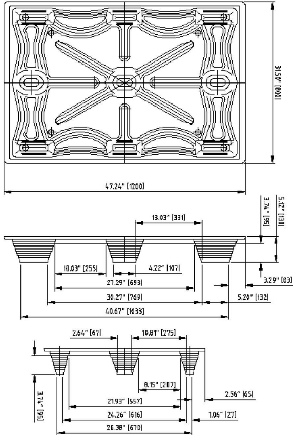
1200mm x 800mm (47.24" x 31.5") PRESSWOOD PALLET
